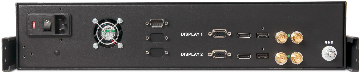
Rear view showing power input and connections
